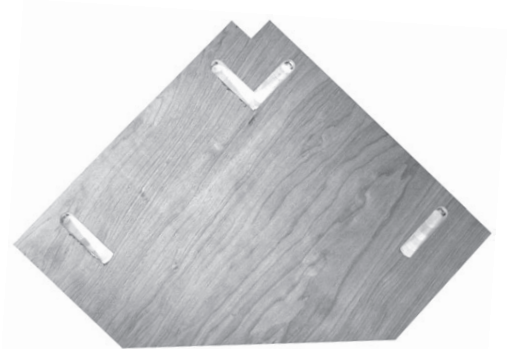
A — Lower Corner Brace — Qty. 1
