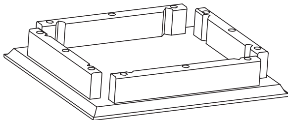
C — Small Top Assembly — Qty. 1
